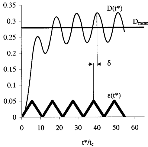
FIG. 8. Deformation and capillary number versus time for \varepsilon_{\max}=0.05 , \lambda=1 and T_o=5.26t_c and A/B=1 .
