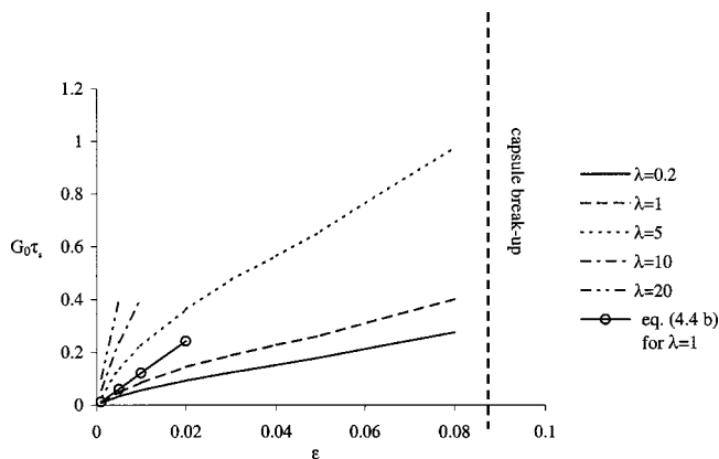
FIG. 4. Dimensionless response time versus capillary number \varepsilon for an initially spherical capsule and for different viscosity ratios \lambda .
