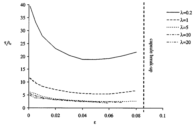
FIG. 5. Intrinsic response time versus capillary number \varepsilon for an initially spherical and for different viscosity ratios \lambda .
