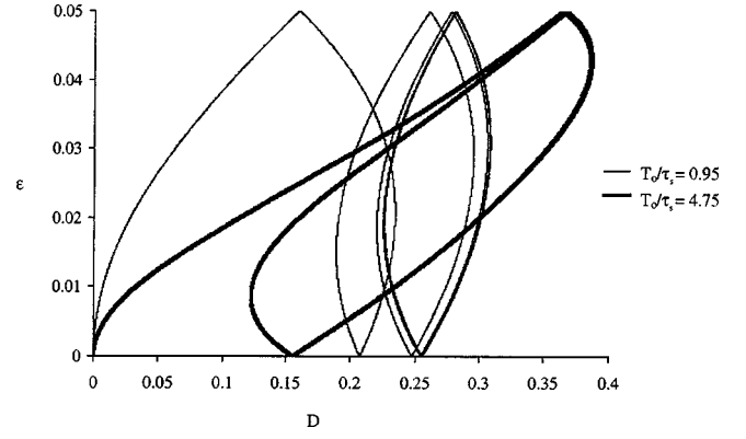
FIG. 11. Capillary number \epsilon versus deformation for a capsule with viscosity ratio \lambda = 1 , for \epsilon_{\max} = 0.05 , T_0/\tau_s = 0.95 , and T_0/\tau_s = 4.75 ( A/B = 1 ).
