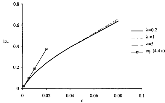
FIG. 3. Steady-state deformation versus \varepsilon for an initially spherical capsule and for different viscosity ratio \lambda .
