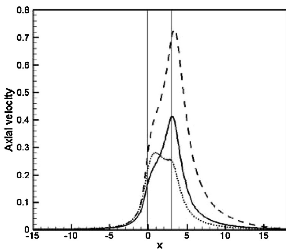
Fig. 3. Axial velocity along r = 0 for pressure driven flow “Case I” at 300 K (solid line) and “Case II” 80 K (dashed line) as well as mixed flow “Case IV” (dotted line), with P_A = 0.3 Pa and P_B/P_A = 0.2 .
